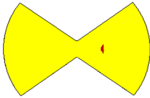
Fig. 3. Antenna I with an off-center coaxial feed.
