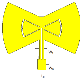
Fig. 6. Antenna IV with a “split-bowtie-shaped” slot and “double-line feed”.
