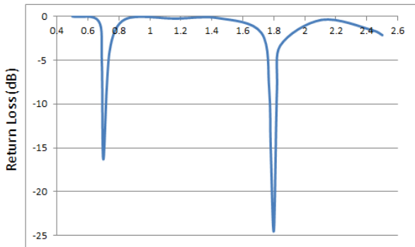
Fig. 8. Return loss versus frequency of antenna II.
